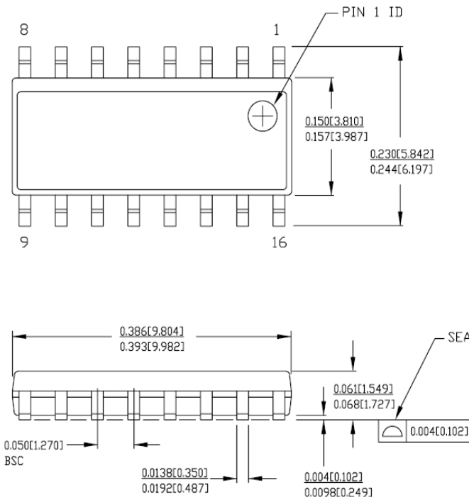
Figure 5. 16-Pin (150-Mil) SOIC (51-85068)
